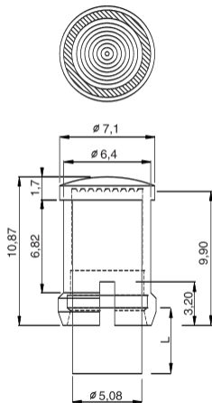
Dimensions in mm (typical)
