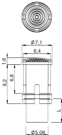
Dimensions in mm (typical)
