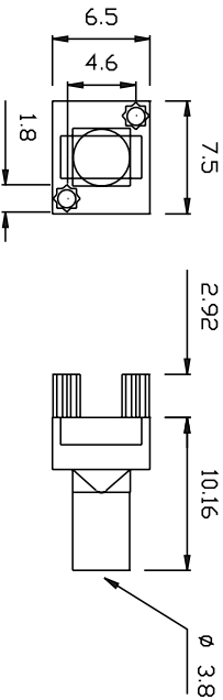
Dimensions in mm (typical)
