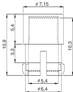
Dimensions in mm (typical)
