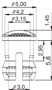
Dimensions in mm (typical)
