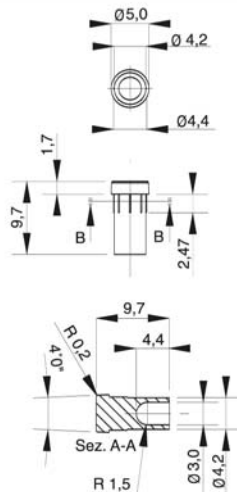
Dimensions in mm (typical)
